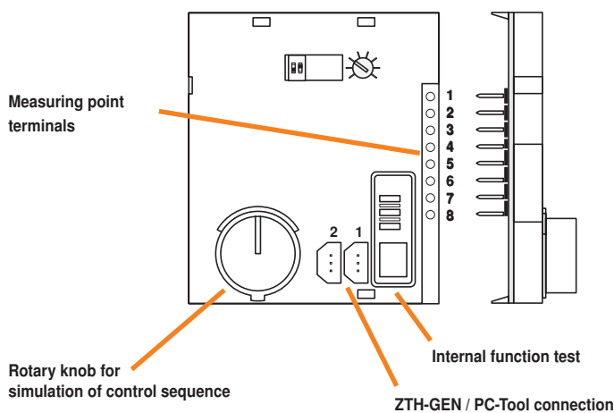
ZTH-GEN / PC-Tool connection
